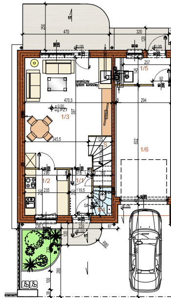
PARTER wariant 2
